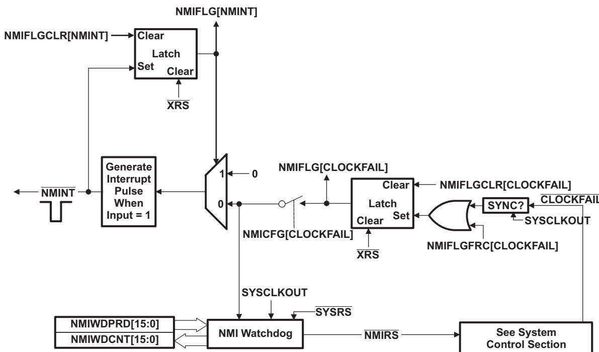
Figure 2-15. NMI-Watchdog
